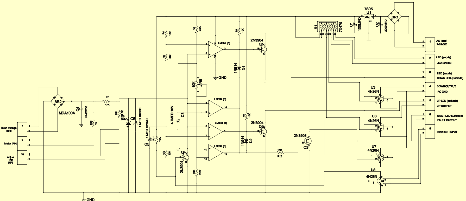
Figure 12.3 – Interface from modified plasma cutter to Mach2 parallel port
